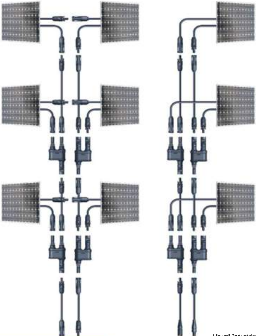
Connectors application diagram
